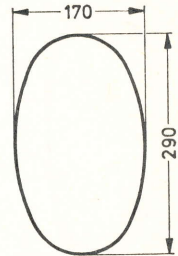
E290x170.1 Standard
