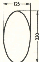
E 230 × 125.1 Standard
