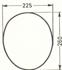
E 260 x 225.1 Standard
