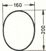
E 200 x 160.1 Konkav
